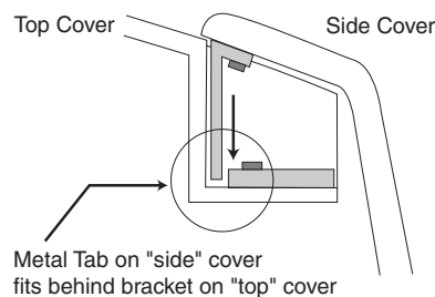
Figure 2 Side and Top Cover Clasp
