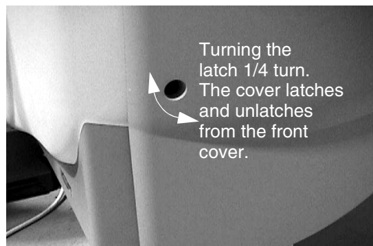
Figure 1 Side Cover Latches
