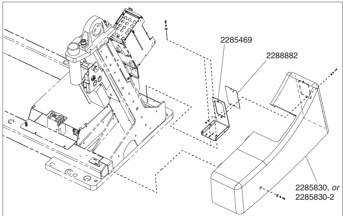
Figure 5 Installation of new right base cover
