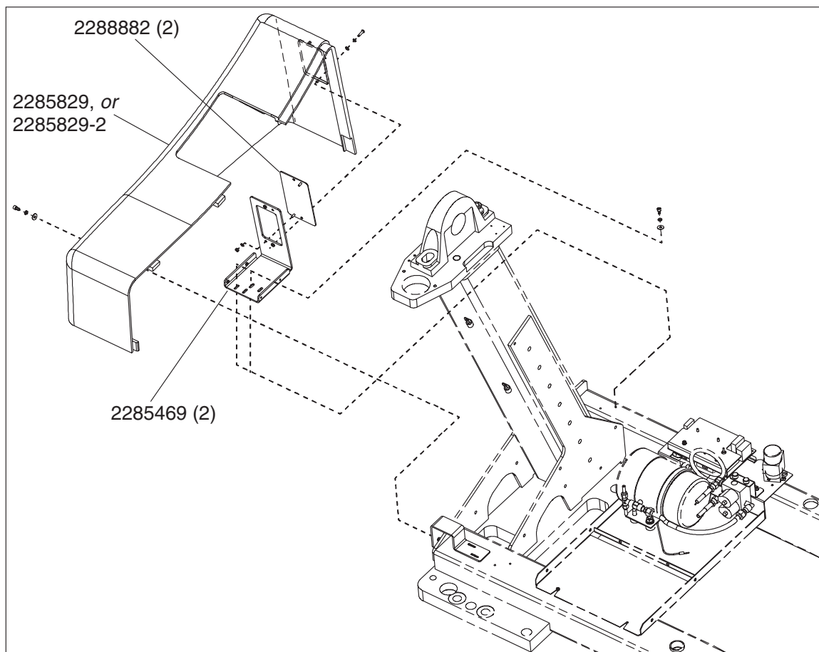
Figure 4 Installation of new left base cover
