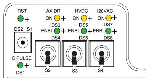
Figure 3 STC Power Switches
